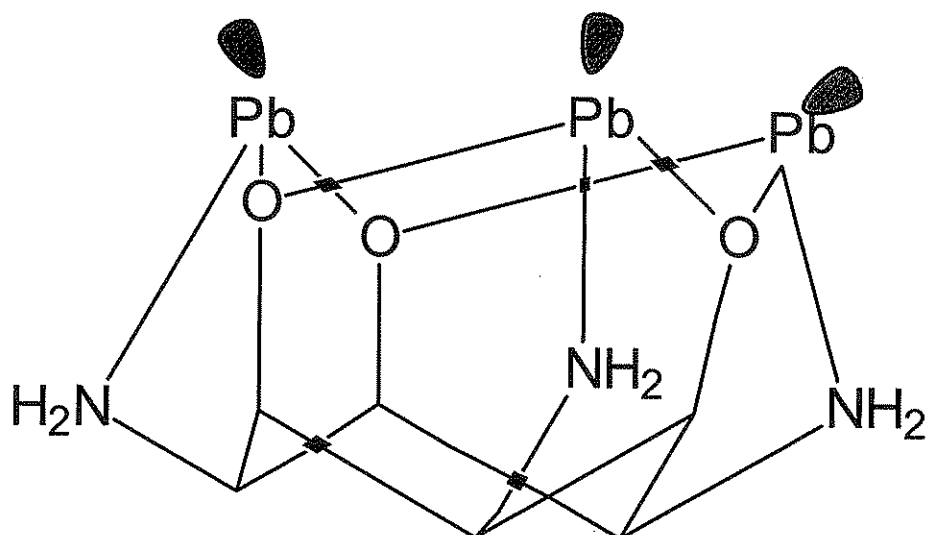
FIGURE 7. Figure showing the stereochemically active 2s lone pair on Pb^{2+} in the compound 1,3,5-triamino-1,3,5-trideoxy- cis -inosital.
