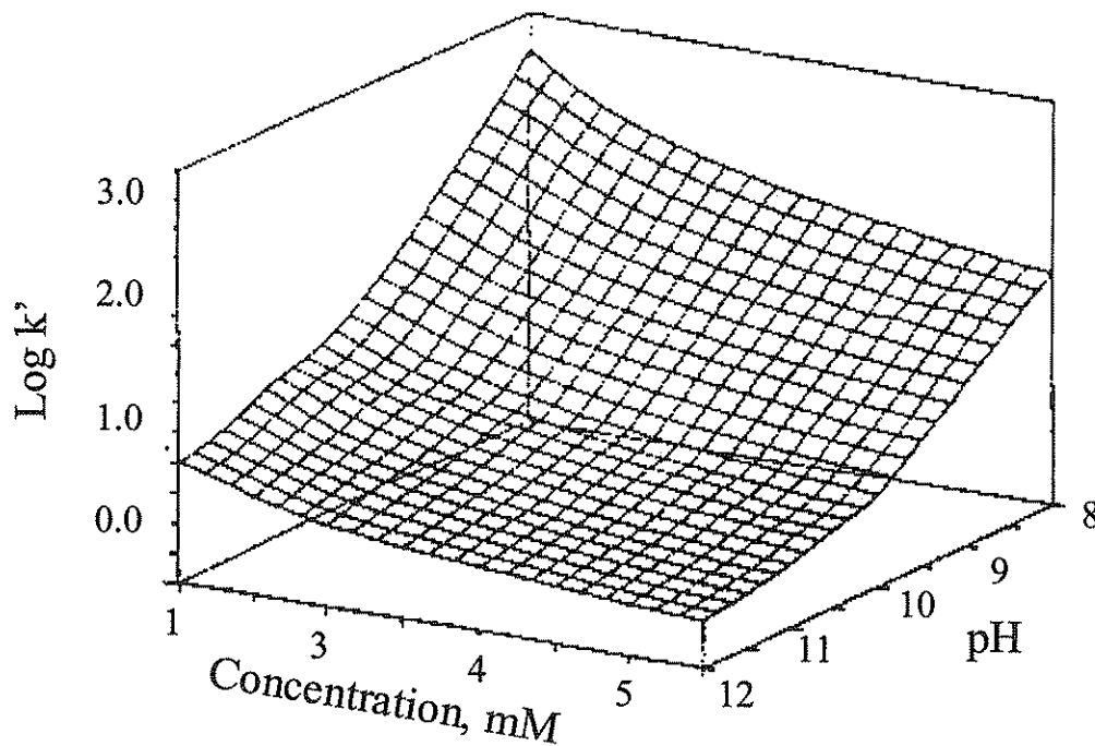
FIGURE 51. Calculated retention surface for the anionic PbEDTA complex eluted with HCO_3^- - CO_3^{2-} buffer (conc. - [HCO_3^-] + [CO_3^{2-}] ). (From P. Hajos, G. Revesz, O. Horvath, J. Peear, C. Sarzanin, J. Chrom. Sci. 1996, 34 , 291.)
