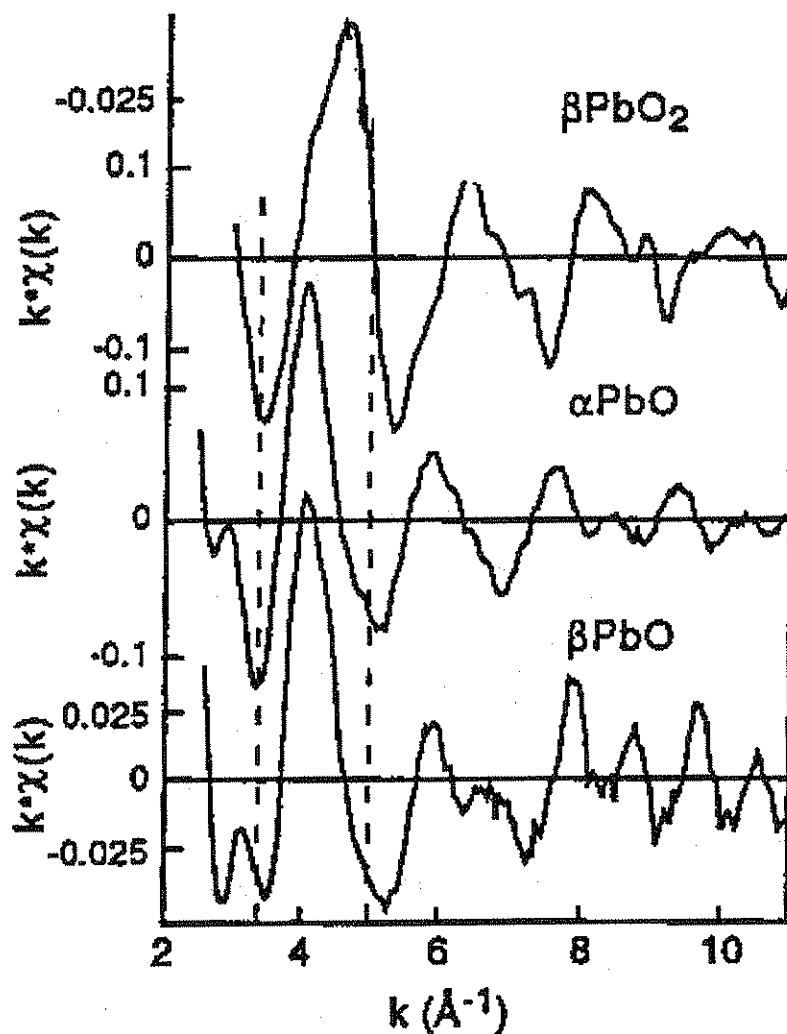
FIGURE 39. When an highly intense radiation source is used (synchrotron), the absorption edge transitions can be resolved into fine structure, which is the result of valence shell electron bonding. This figure illustrates the difference observed between \alpha and \beta PbO. (From A. Manceau, M.-C. Boisset, G. Sarret, J.-L. Hazemann, M. Mench, P. Cambier, and R. Prost Environ. Sci. Tech. 1996, 30, 1540–1552.)
