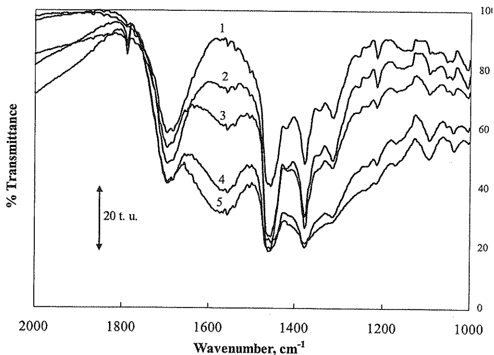
FIGURE 42. The binding of lead to the carboxyl groups on EDTA (see Figure 12) changes the single/double bond character of the carbonyl bond of the COO functional group. Deprotonation and stabilization of the carboxylate group with a metal ion maximizes resonance enhancing the single bond character of the carbonyl group, lowering the frequency of the vibration. Infrared spectra of PbEDTA and EDTA mixtures, the molar ratio of PbEDTA being (a) 0; (b) 0.25; (c) 0.5; (d) 0.75, and (e) 1.0. Each of the mixtures has a total of 10 \mu\text{mol} of ligand. (From S. Dragan and A. Fitch, J. Chem. Ed. , 1998, 75 , 1018–1021.)
