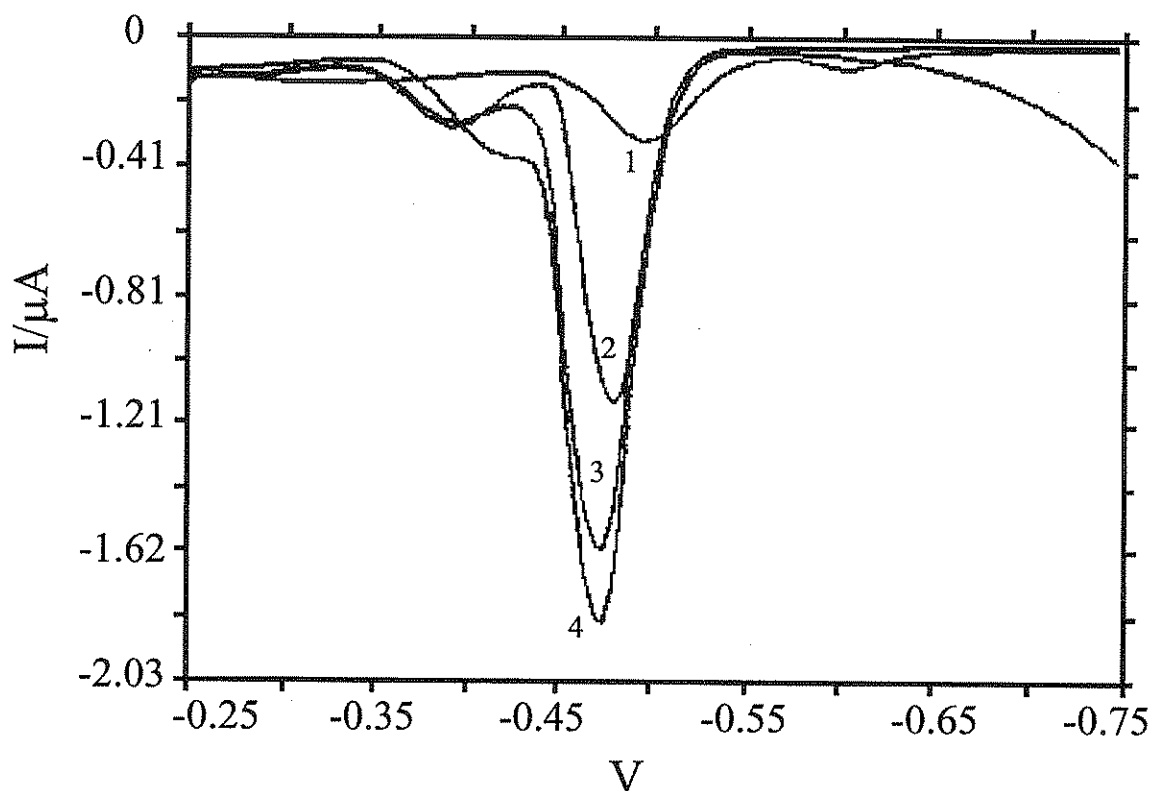
FIGURE 17. Square wave anodic stripping voltammogram of 10 ppb Pb and 150 ppb In from a solution containing 1.2 M HCl and variable concentrations of NaBr (0.0; 1.0, 1.5, and 2.0 M). As the bromide concentration is increased, the peak sharpens and shifts to more positive potentials. (From Liu, T. Z., D. Lai, and J. D. Osterloh, Anal. Chem. , 1997, 69 , 3539–3543.)
