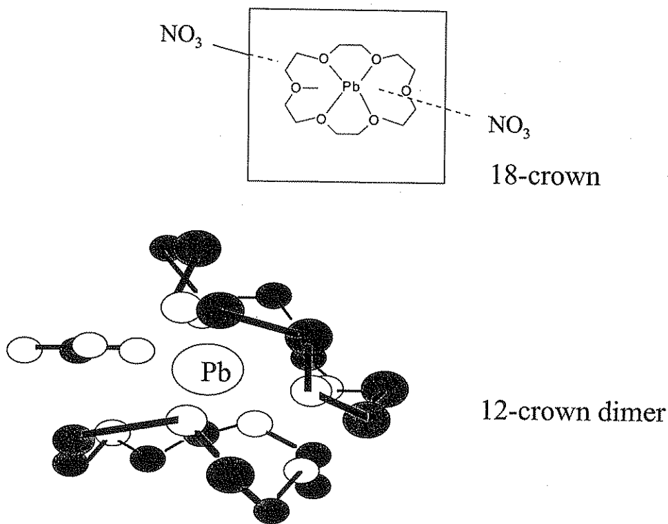
FIGURE 9. (A) 18-crown ether has been used as a lead ionophore but does not exhibit stereochemical activity of the 2s lone pair on Pb 2+ . In this figure the Pb(18-crown-6) cation and its 2 NO 3 - anions are viewed almost perpendicularly (M. G. B. Drew, D. G. Nicholson, I. Sylte, and A. K. Vasudevan, Acta Chem. Scan. 1992, 46, 396-398). (B) The dimeric 12 crown ether used as a lead ionophore does exhibit stereochemical activity of the 2s lone pair on Pb 2+ . (D. G. Nicholson, I. Sylte, A. K. Vasudevan, and L. J. Saethre, Acta Chem. Scan. 1992, 46, 358-362.) One site is occupied by the lone pair and another by NO 3 - .
