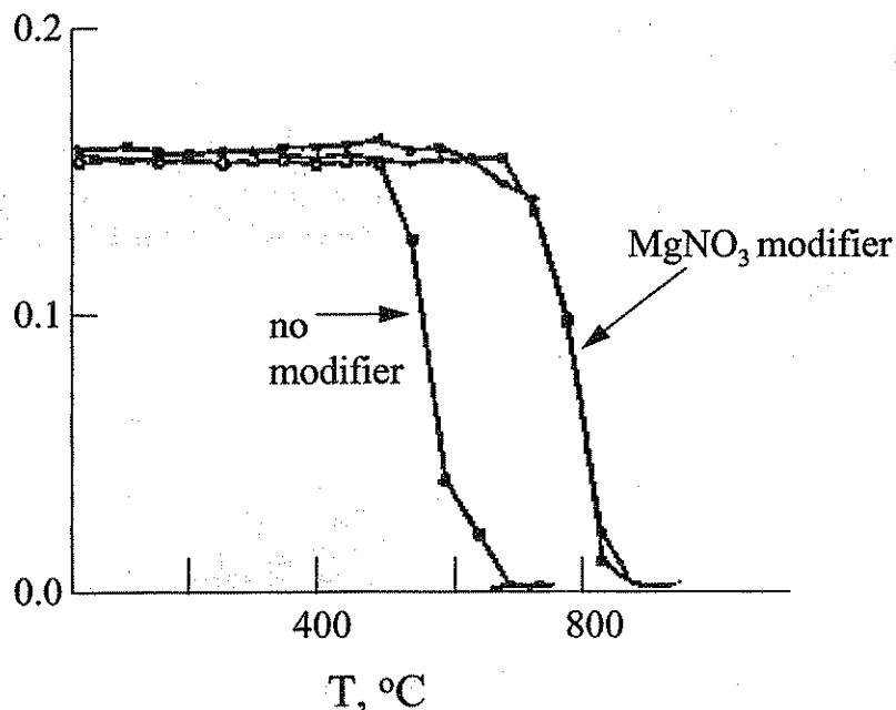
FIGURE 22. The temperature at which the lead is volatilized as a gas is modified by the presence of the nitrate (see Figure 4), which produces lead oxide. In normal solution lead may volatilize at very low temperatures due to the presence of halides. The presence of the oxide raises the temperature of volatilization. (From A. Deval and J. Sneddon, Microchemical Journal , 1995, 52 , 96–100.)
