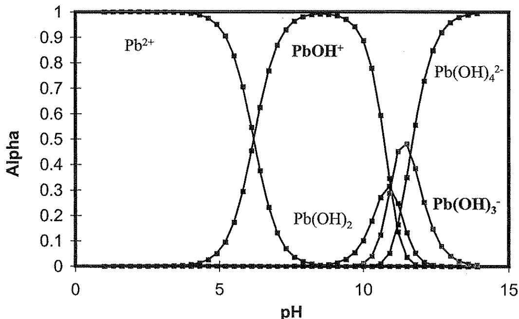
FIGURE 3. Plot of the fraction of lead in various hydroxy forms as a function of pH.
