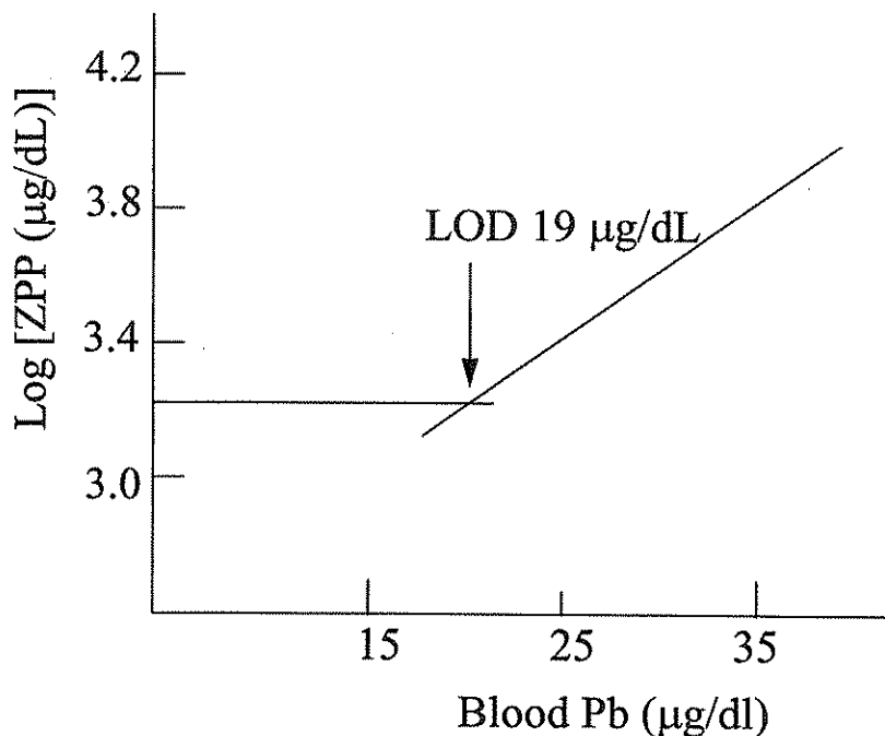
FIGURE 36. The lead dose, zinc protoporphyrin response curve. (From P. B. Hammond, R. L. Bornschein, and P. Sucop, Environmental Research , 1985, 38 , 187–196.)
