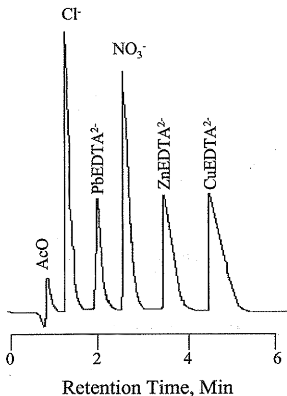
FIGURE 52. Chromatogram of anionic metal-EDTA complexes and simple anions obtained by using carbonate eluent ((conc. [\text{HCO}_3^-] + [\text{CO}_3^{2-}] = 3.5 \text{ mM} , \text{CO}_3^{2-}\text{-HCO}_3 = 2.0/1.5 ). The pH was 10.4, the sample volume was 50 \mu\text{l} , and a conductivity detector was used. (From P. Hajos, G. Revesz, O. Horvath, J. Peear, C. Sarzanin, J. Chrom. Sci. 1996, 34 , 291.)
