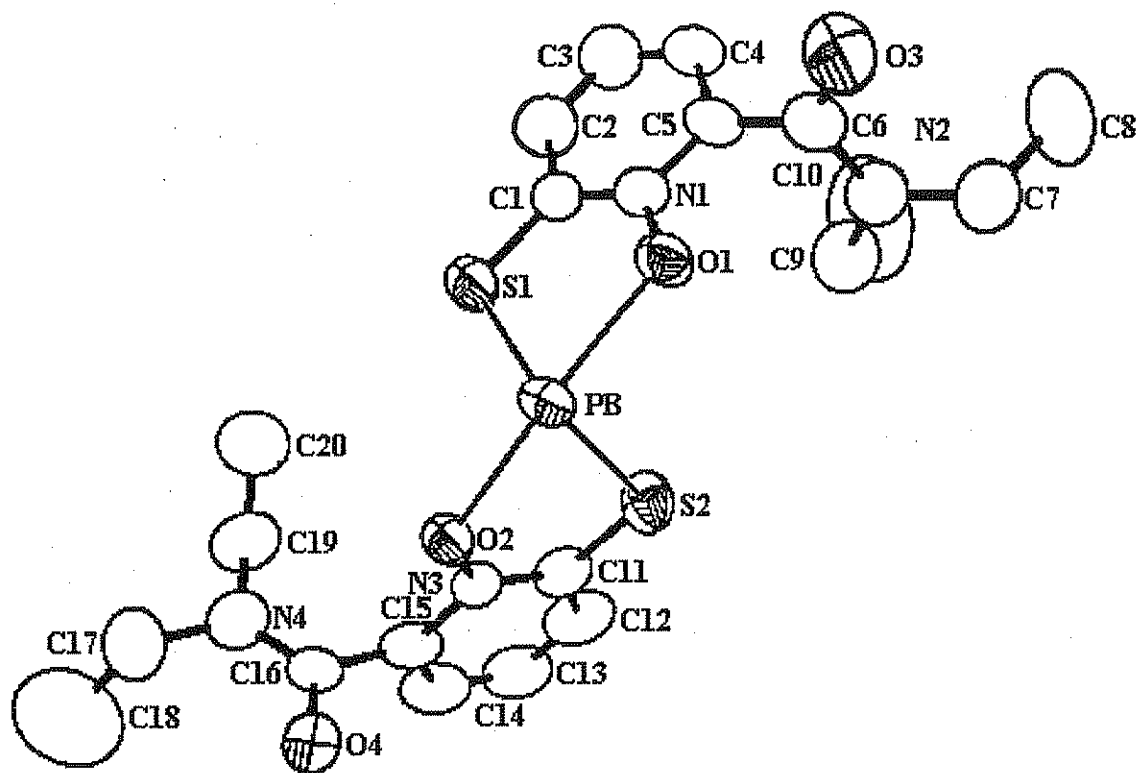
FIGURE 8. Figure showing the stereochemically active 2s lone pair on Pb^{2+} in the compound bis (6-(diethylcarbamoyl)-1-hydroxy-2(1H)-pyridine-2-thionato- O,S )-lead(II). The compound is viewed along the direction occupied by the lone pair on Pb^{2+} . (From Kama Abu-Dari, T. B. Karpishin, and K. N. Raymond, Inorganic Chemistry 1993, 32 , 3052–3055.)
