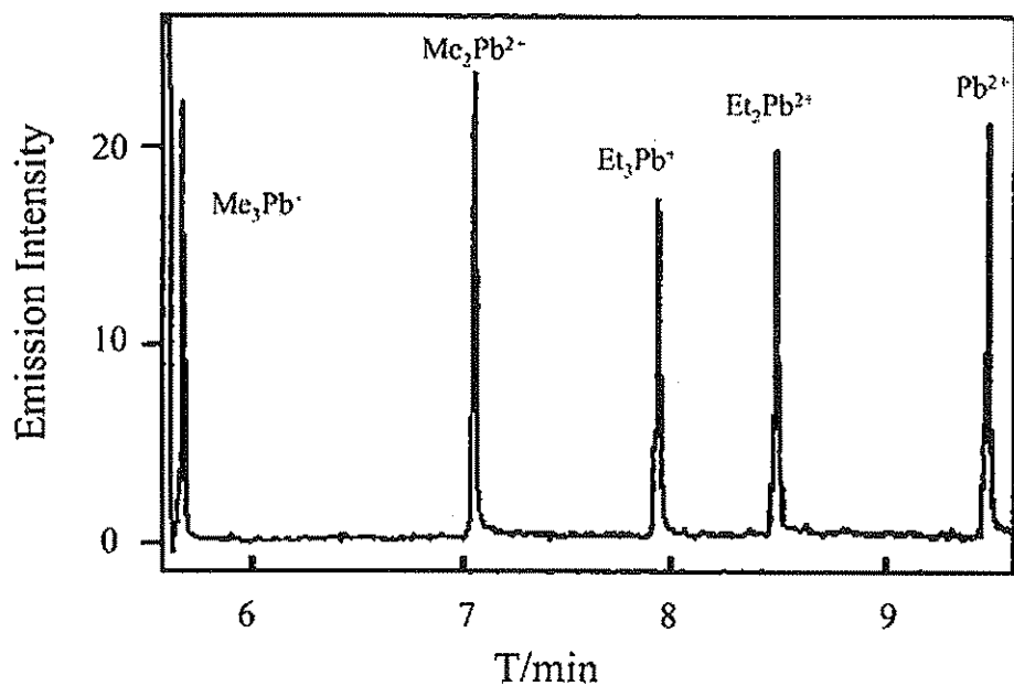
FIGURE 48. Chromatogram obtained using GC-AES of a mixture of propylated organolead standards (3 to 4 pg each) obtained with a Tenxax-packed liner after 60 s solvent venting: (1) \text{Me}_3\text{Pb}^+ ; (2) \text{Me}_2\text{Pb}^{2+} ; (3) \text{Et}_3\text{Pb}^+ ; (4) \text{Et}_2\text{Pb}^{2+} ; and (5) \text{Pb}^{2+} . Emission intensity measured in arbitrary units. (From R. Lobinski, F. C. Adams, J. Anal. Atomic Spectrometry , 1992, 7, 1987.)
