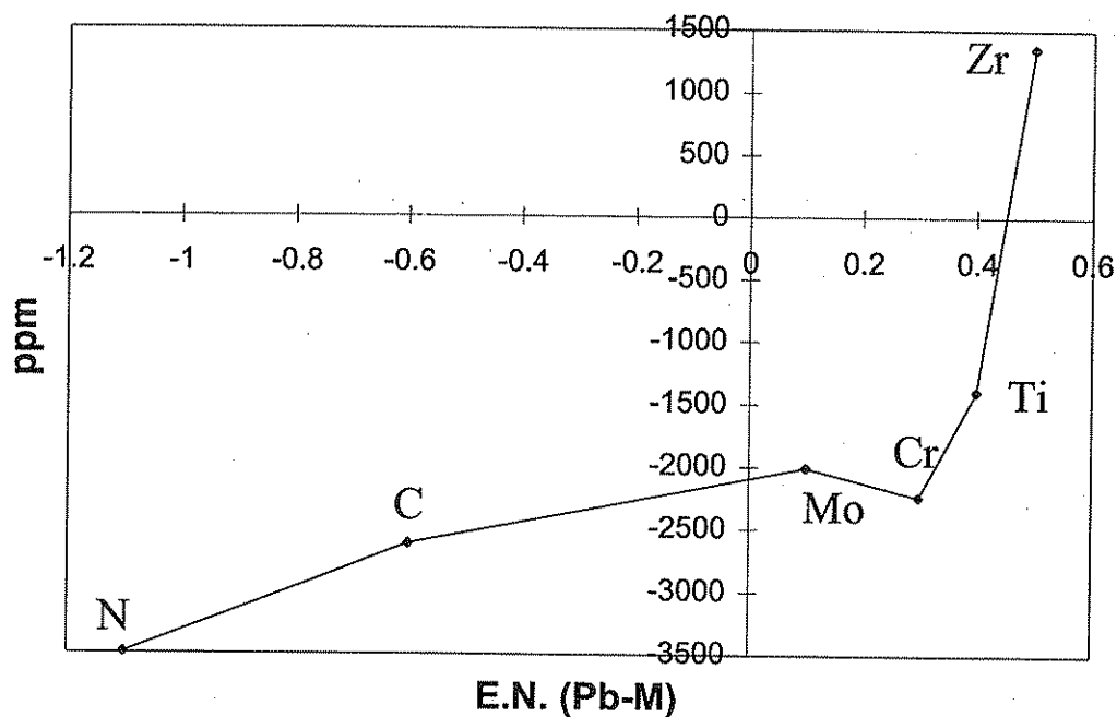
NMR Chemical Shift for \text{PbMxOy}
