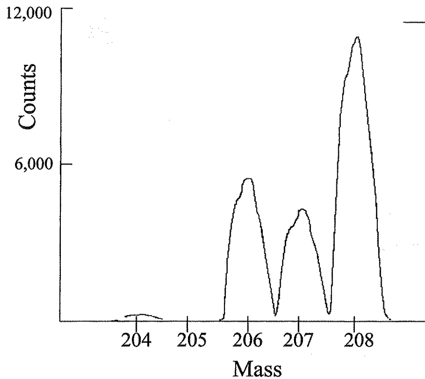
FIGURE 47. A mass spectrum of lead obtained on an ICP-MS showing the four isotope peaks associated with lead.
